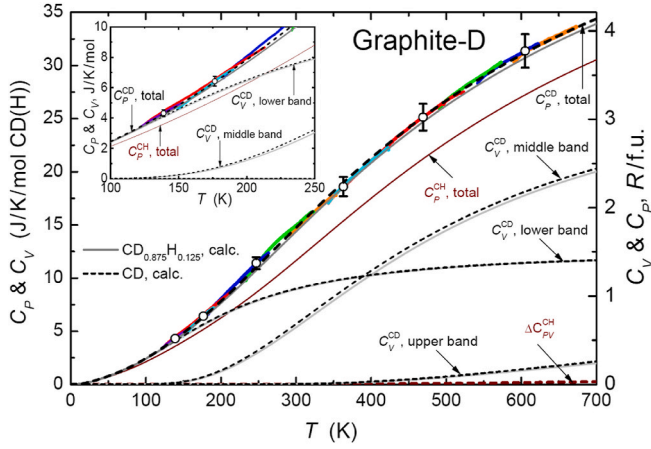
Fig. 13. Temperature dependence of the experimental heat capacity of graphite deuteride with the composition CD_{0.91}H_{0.09} (thick colored curves) and calculated dependences of the heat capacity of the graphane II phases of deuterides CD (dashed black curves) and CD_{0.875}H_{0.125} (solid grey curves). The dependences of the calculated heat capacity at constant pressure are obtained from the corresponding C_V(T) dependences by adding the “ \Delta C_{pV}^{CH} ” difference determined for the graphite hydride.
