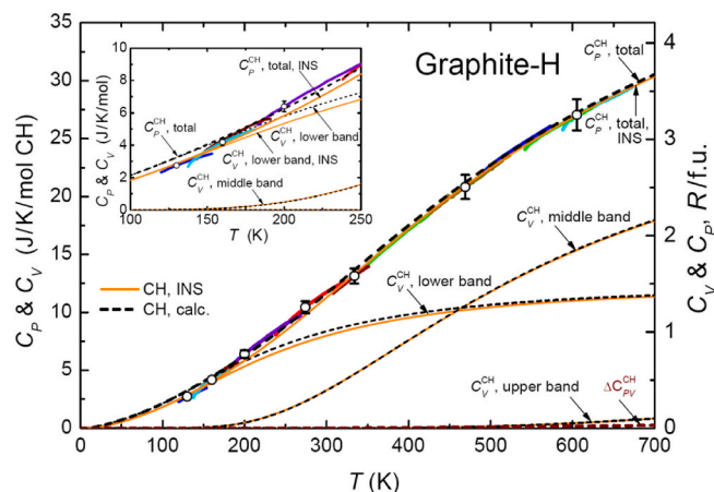
Fig. 12. Temperature dependences of the heat capacity of graphite hydride determined experimentally (thick colored curves) and those calculated from the INS-derived g_{\text{exp}}(E) (thin orange curves). Dashed black curves show the heat capacity of the graphane II phase of graphite hydride resulting from the g_{\text{calc}}(E) calculated by DFT-LDA. The curves labeled “ C_p^{\text{CH}} , total” and “ C_p^{\text{CH}} , total INS” are obtained by adding the difference labeled “ \Delta C_{pV}^{\text{CH}} ” to the corresponding calculated dependences of the total C_V(T) . (For interpretation of the references to color in this figure legend, the reader is referred to the Web version of this article.)
